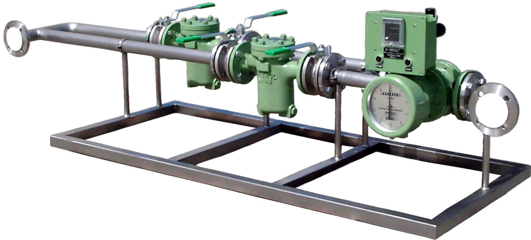
1" METERING SKID WITH PNEUMATIC PRESET COUNTER AND TWO STRAINERS IN PARALLEL
