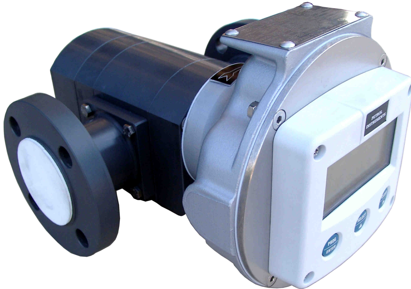
2" SINGLE CASE PD FLOW METER IN PVC WITH I.S. TOTALIZER AND FLOWRATE INDICATOR
